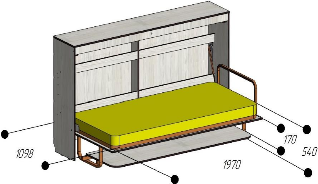
THE WALLBED IS UNFOLDED
