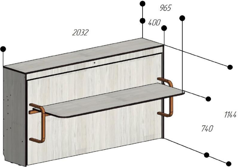
THE WALLBED IS FOLDED
